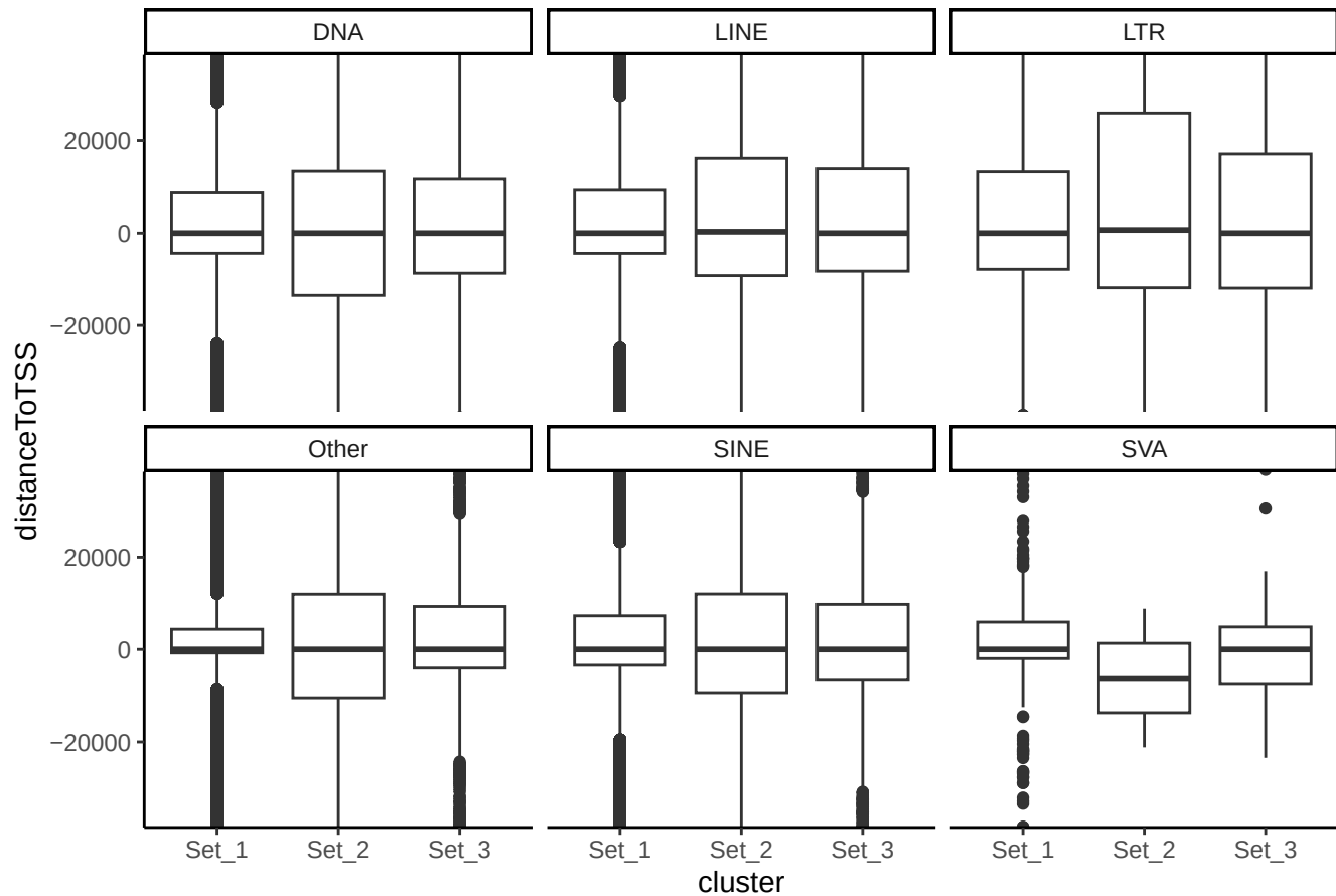
Distance to TSS by class in H3K27ac of overlapping ROIs
